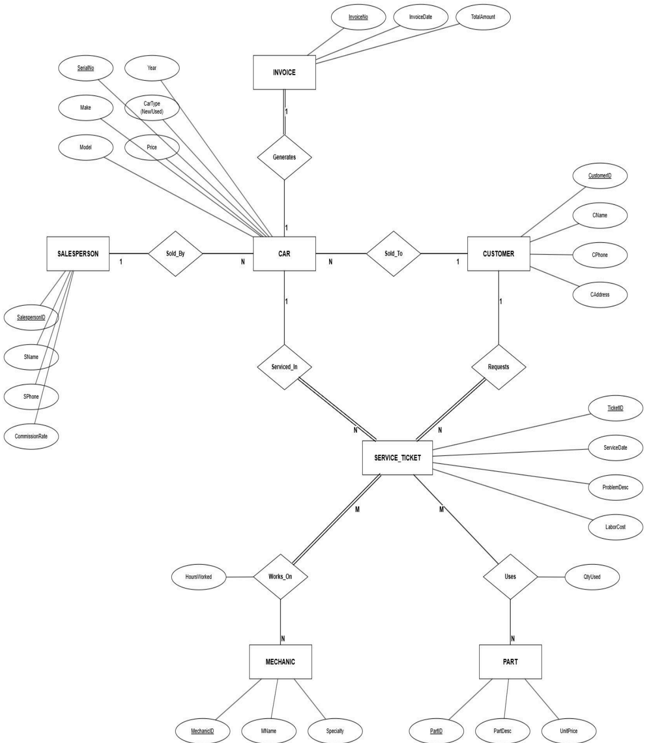
Car Dealership - ER Diagram (Chen Notation)
