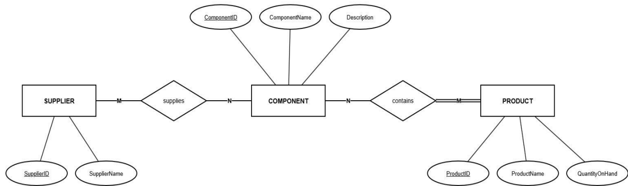
Manufacturer ER Diagram (Chen notation)
